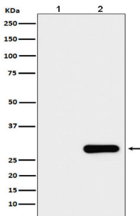
Western blot analysis of GFP protein expression in (1) 293T cell lysate; (2) 293T cell transfected with GFP protein lysate.
