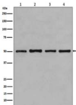
Western blot analysis of beta Tubulin expression in (1) MCF-7 cell lysate; (2) COS-1 cell lysate; (3) Jurkat cell lysate; (4) HeLa cell lysates
